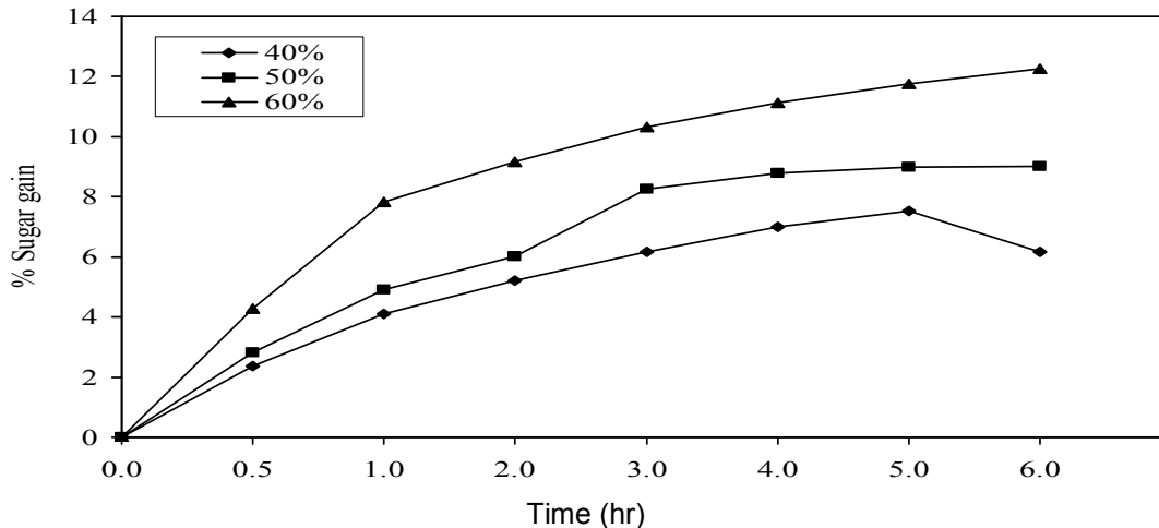
Fig. 2. Influence of different sugar solution concentration at 40°C on % sugar gain (SG) of pineapple slices of 10mm thickness
