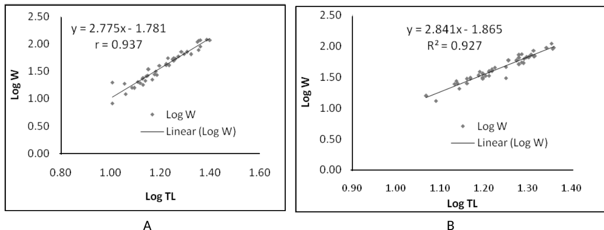
Fig. 2. Logarithmic relationship between total length and body weight of (A) male and (B) Female, G. giurus
